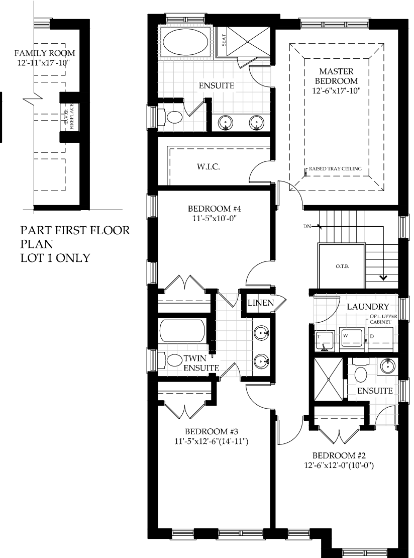
SECOND FLOOR PLAN ELEVATION 'A' 1370.91 S.F.
