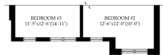
SECOND FLOOR PART PLAN ELEVATION 'B' 1363.86 S.F.
