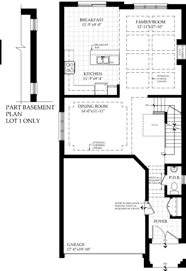
FIRST FLOOR PLAN ELEVATION 'A' 991.47 S.F. COVERAGE 1396.16 S.F. INCL. PORCH
