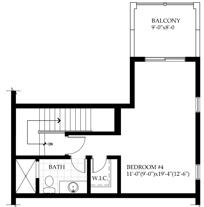
THIRD FLOOR PLAN ELEVATION 'A'
